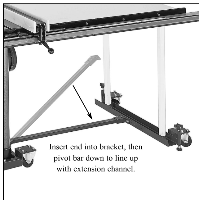
Figure 7. Attaching extension bar.
