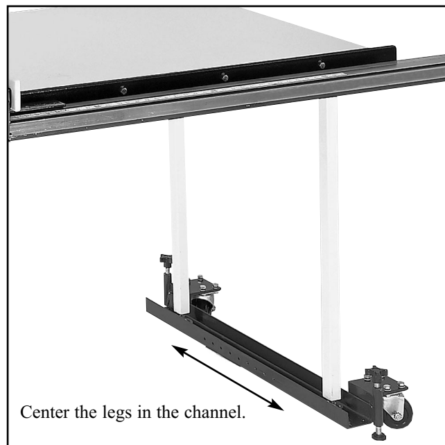
Figure 6. Extension table legs on channel.
