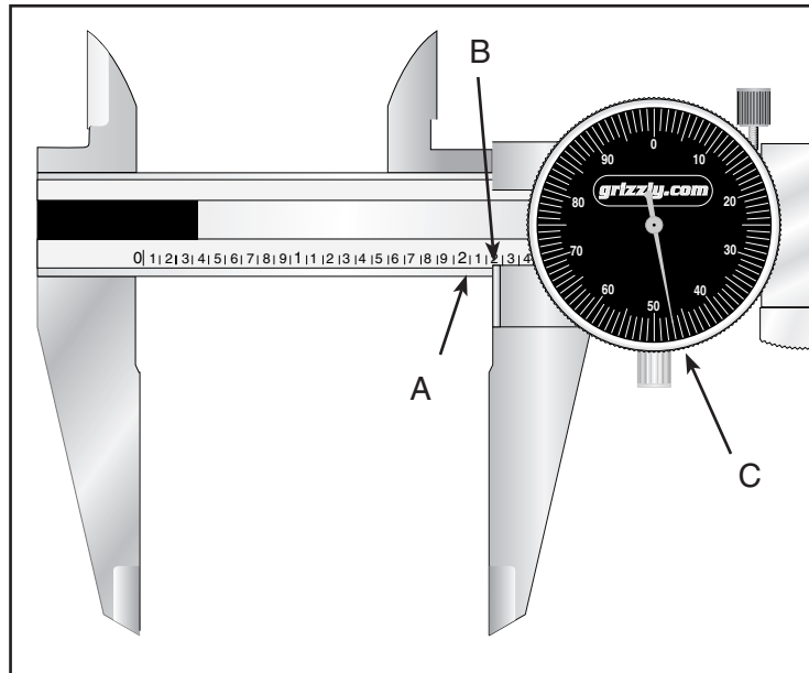
Figure 2. Measuring 2.147".
