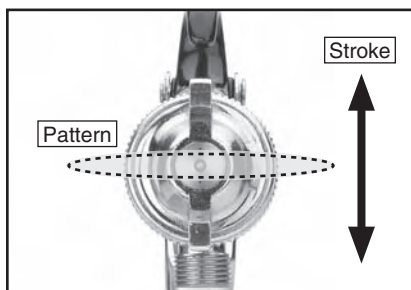
Figure 12. Set up for vertical stroke direction with horizontal fan pattern.
