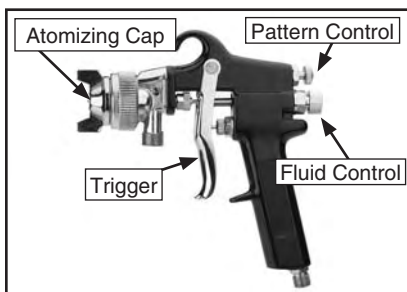
Figure 8. Controls.
