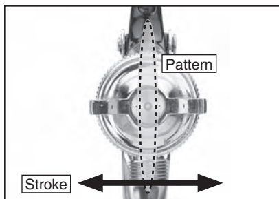
Figure 13. Set up for horizontal spray stroke with vertical fan pattern.
