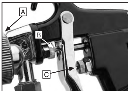
Figure 22. Lubrication points.
