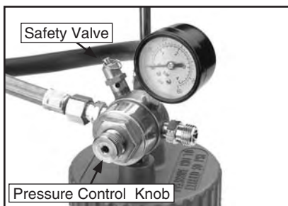
Figure 9. Pressure cup controls.
