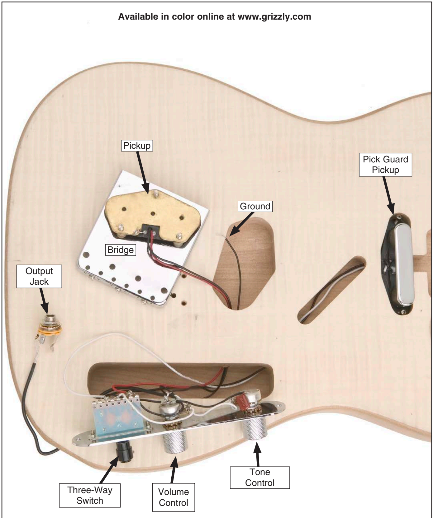
Figure 55. Model H8070 overall wiring.
