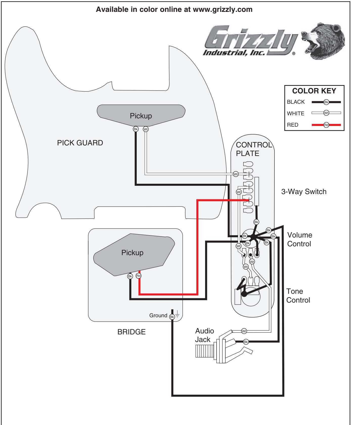
Figure 56. Model H8070 wiring diagram.
