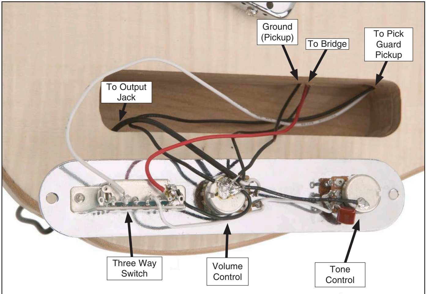
Figure 53. Control plate wiring.
