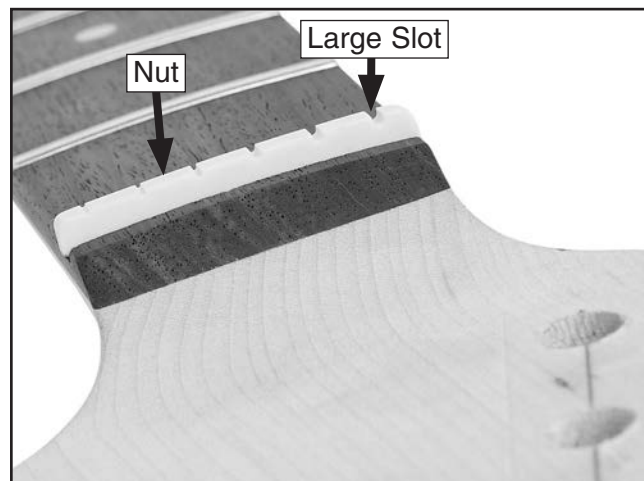
Figure 27. Nut installed.
