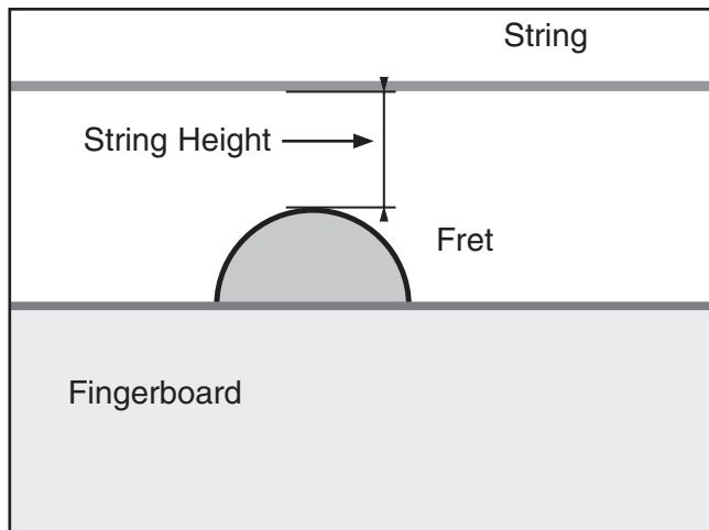
Figure 34. String height measurement.
